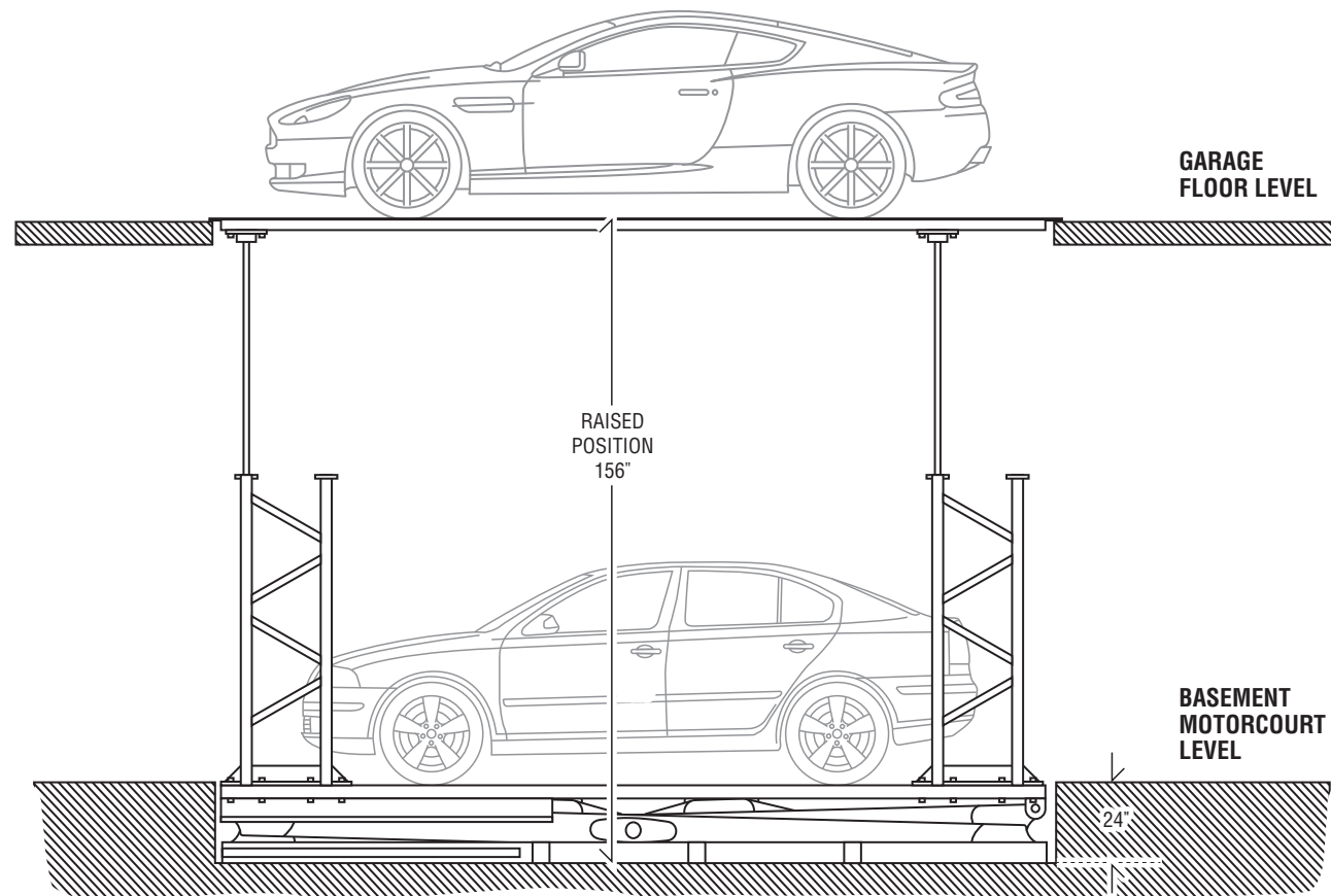
FIG. 10 LOWERED POSITION
