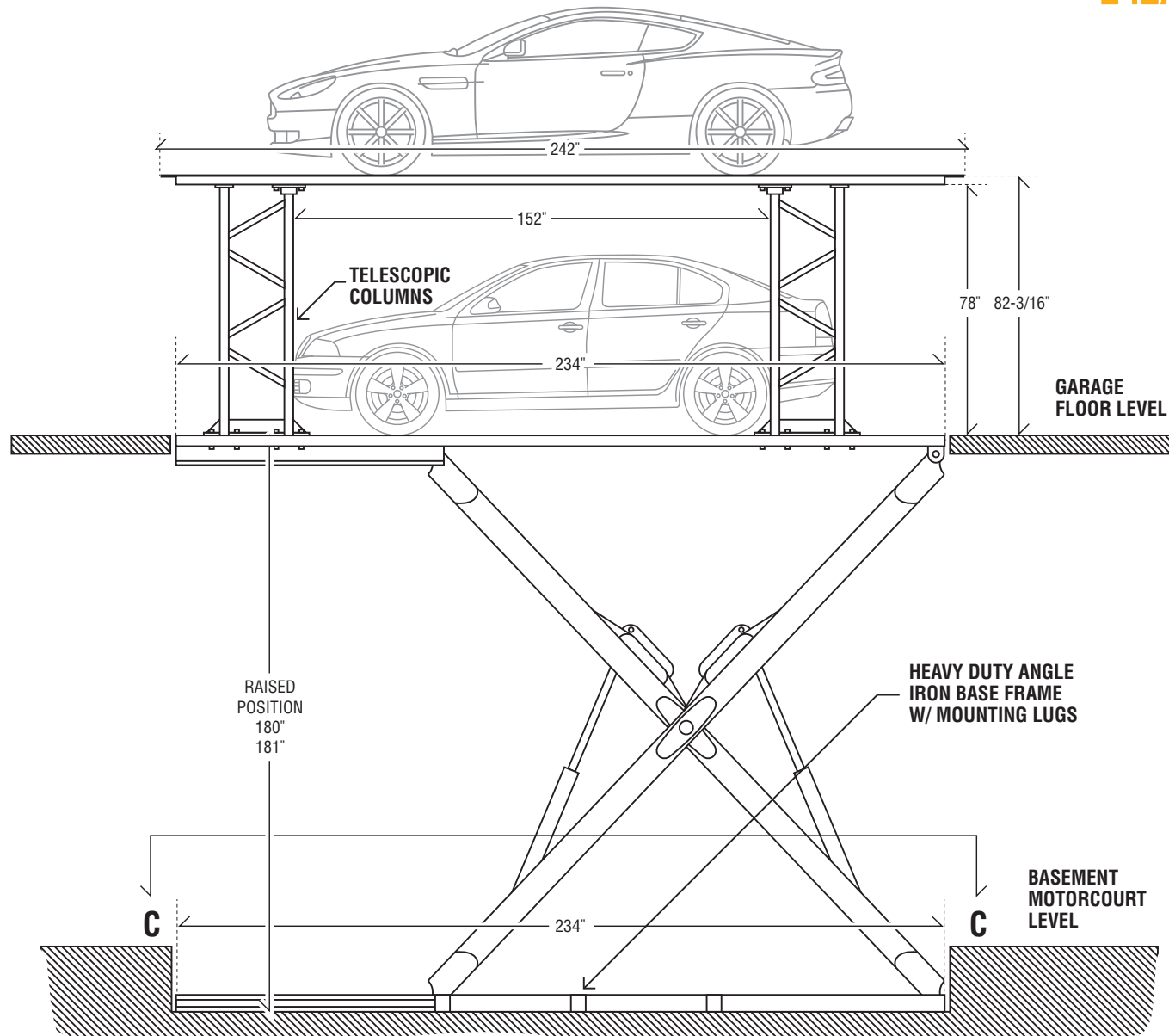
FIG. 13 RAISED POSITION
